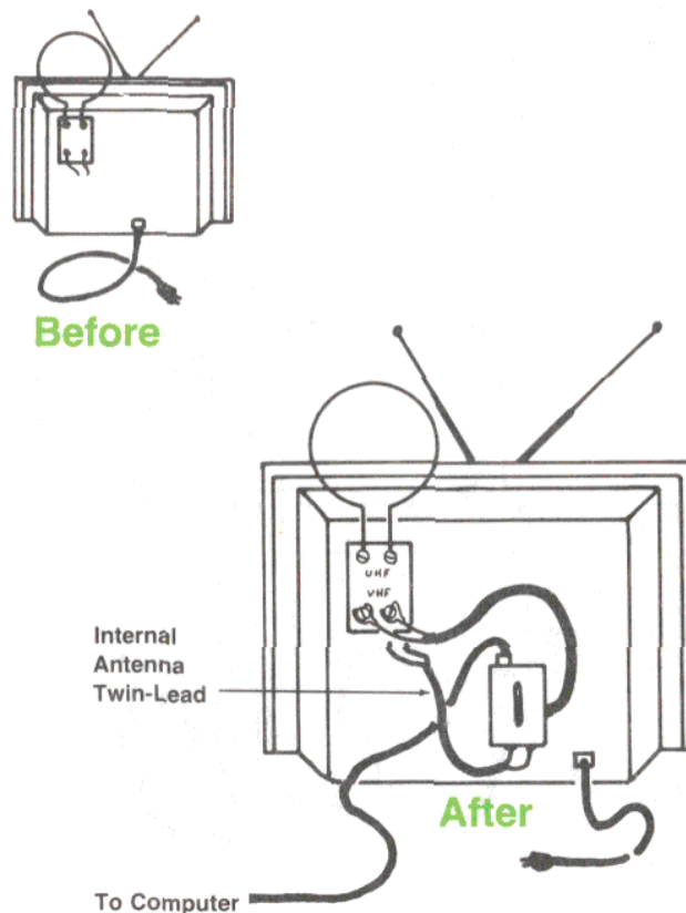
Figure 2. Rear View of TV with Screw Terminals and Internal Antenna.
