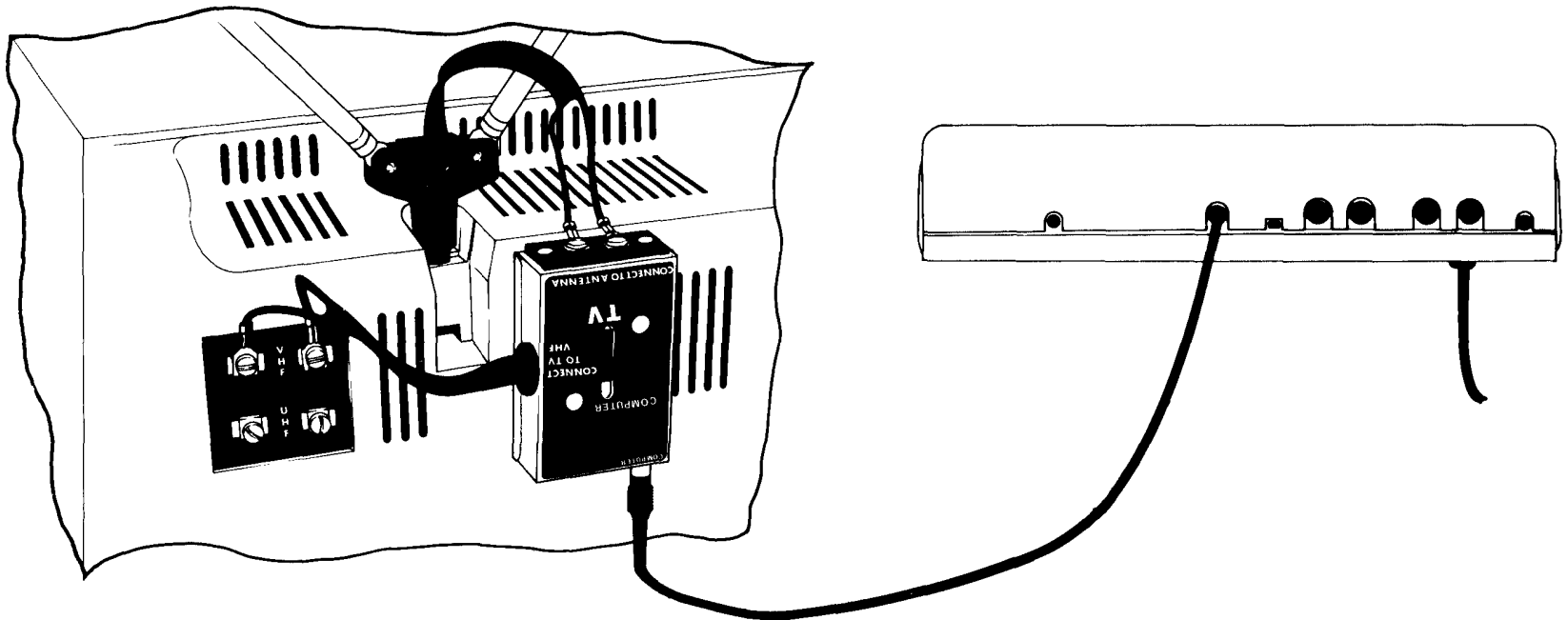
Figure 7. Connection of the Computer to the Switchbox.
