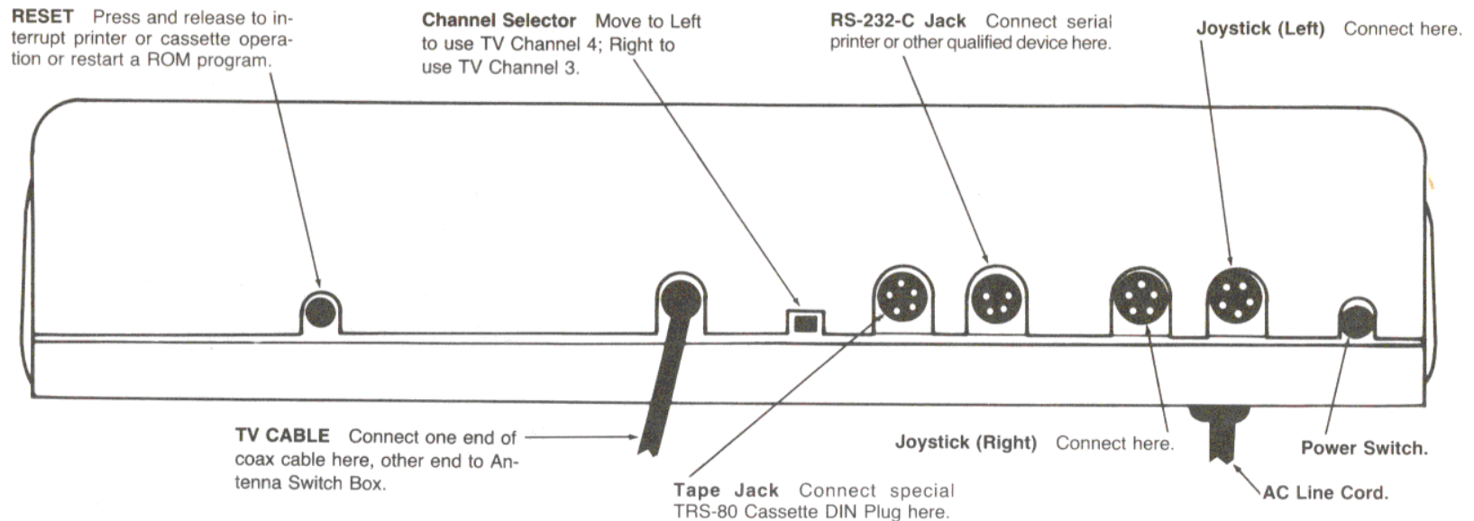
Figure 9. Computer Controls and Connections.
